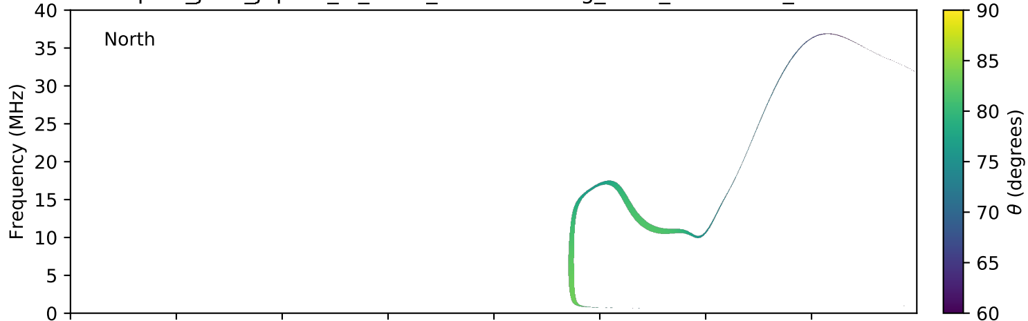
expres_juno_jupiter_io_isaac_lossc-wid1deg_3kev_20170112_v01.cdf
