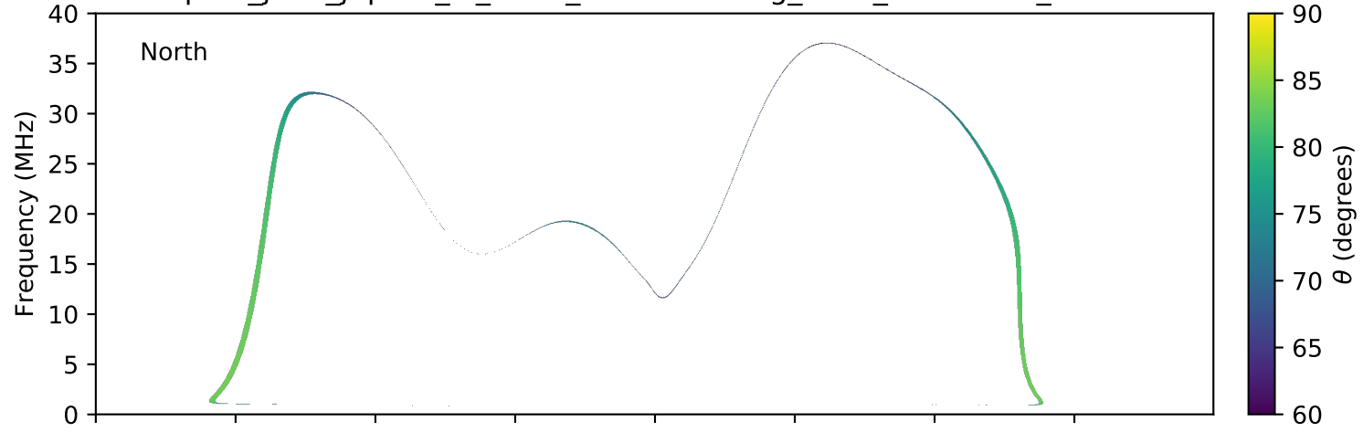
expres_juno_jupiter_io_isaac_lossc-wid1deg_3kev_20170109_v01.cdf
