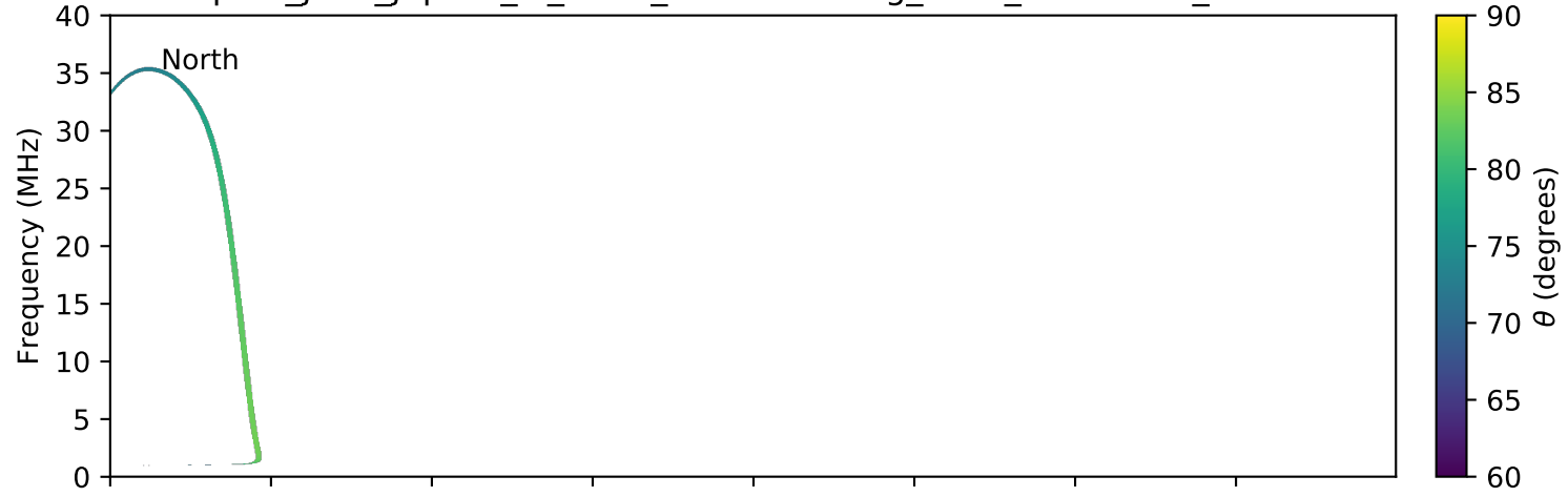
expres_juno_jupiter_io_isaac_lossc-wid1deg_3kev_20170108_v01.cdf
