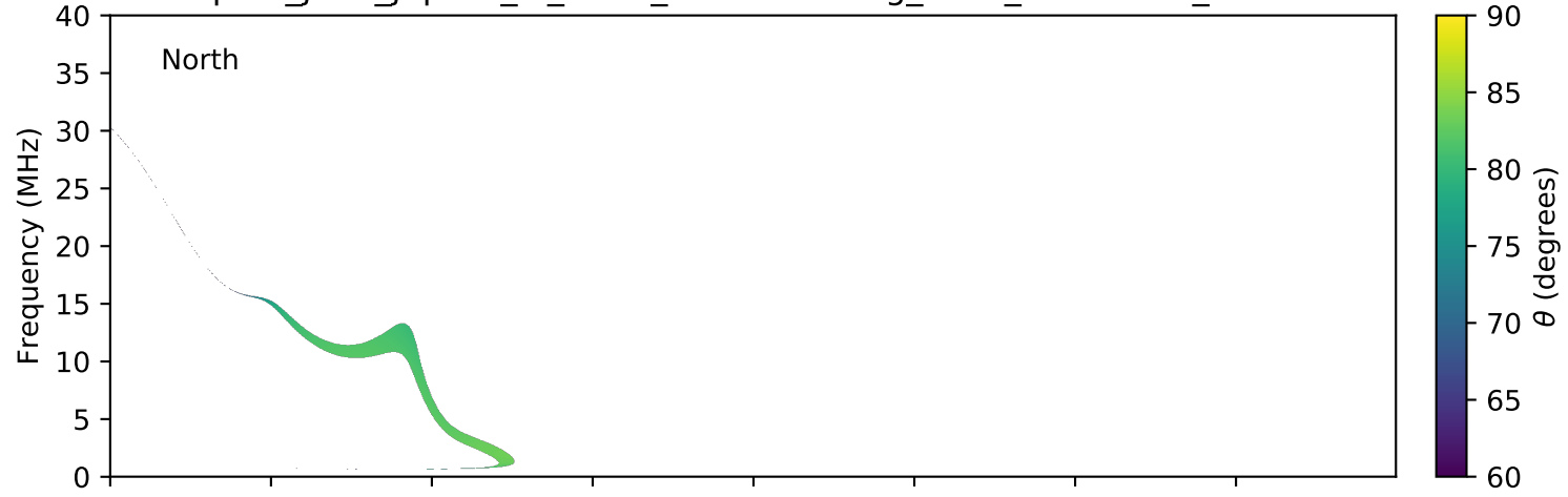
expres_juno_jupiter_io_isaac_lossc-wid1deg_3kev_20170106_v01.cdf
