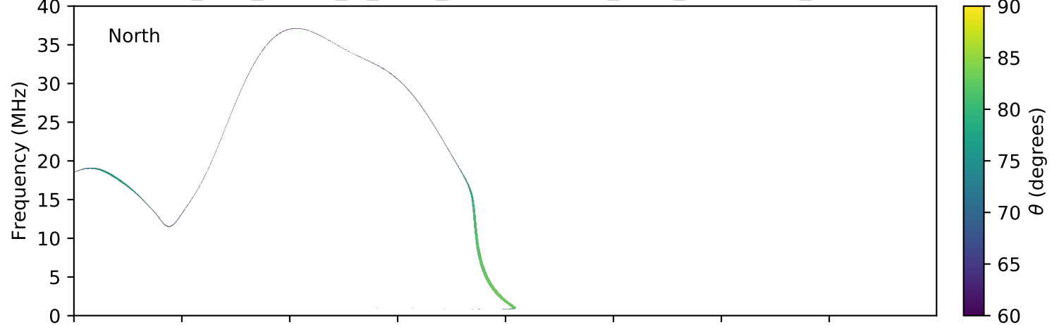
expres_juno_jupiter_io_isaac_lossc-wid1deg_3kev_20170104_v01.cdf
