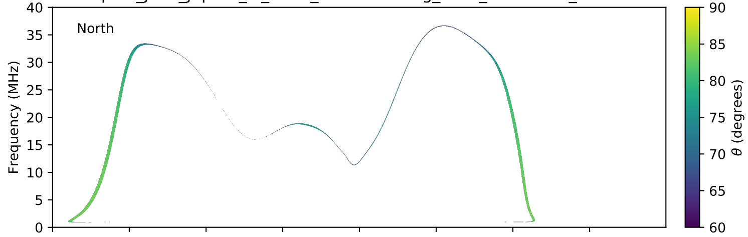
expres_juno_jupiter_io_isaac_lossc-wid1deg_3kev_20170102_v01.cdf
