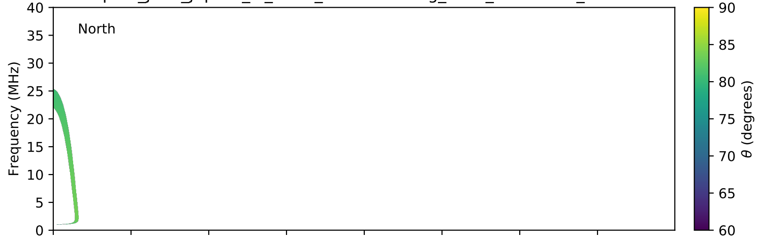
expres_juno_jupiter_io_isaac_lossc-wid1deg_3kev_20170101_v01.cdf
