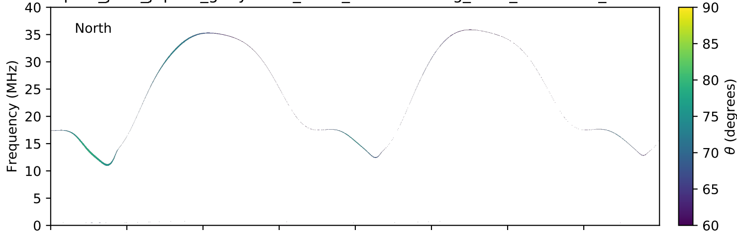
expres_juno_jupiter_ganymede_isaac_lossc-wid1deg_3kev_20170130_v01.cdf
