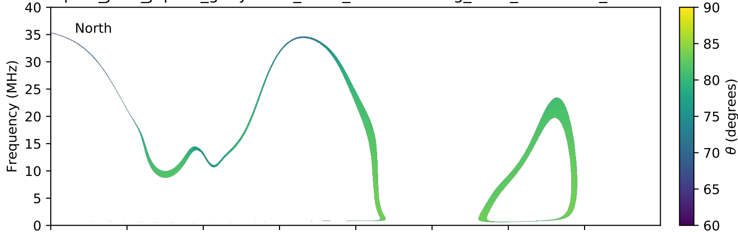
expres_juno_jupiter_ganymede_isaac_lossc-wid1deg_3kev_20170125_v01.cdf
