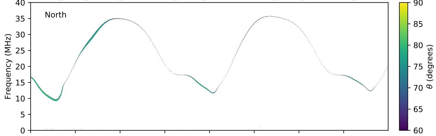
expres_juno_jupiter_ganymede_isaac_lossc-wid1deg_3kev_20170123_v01.cdf
