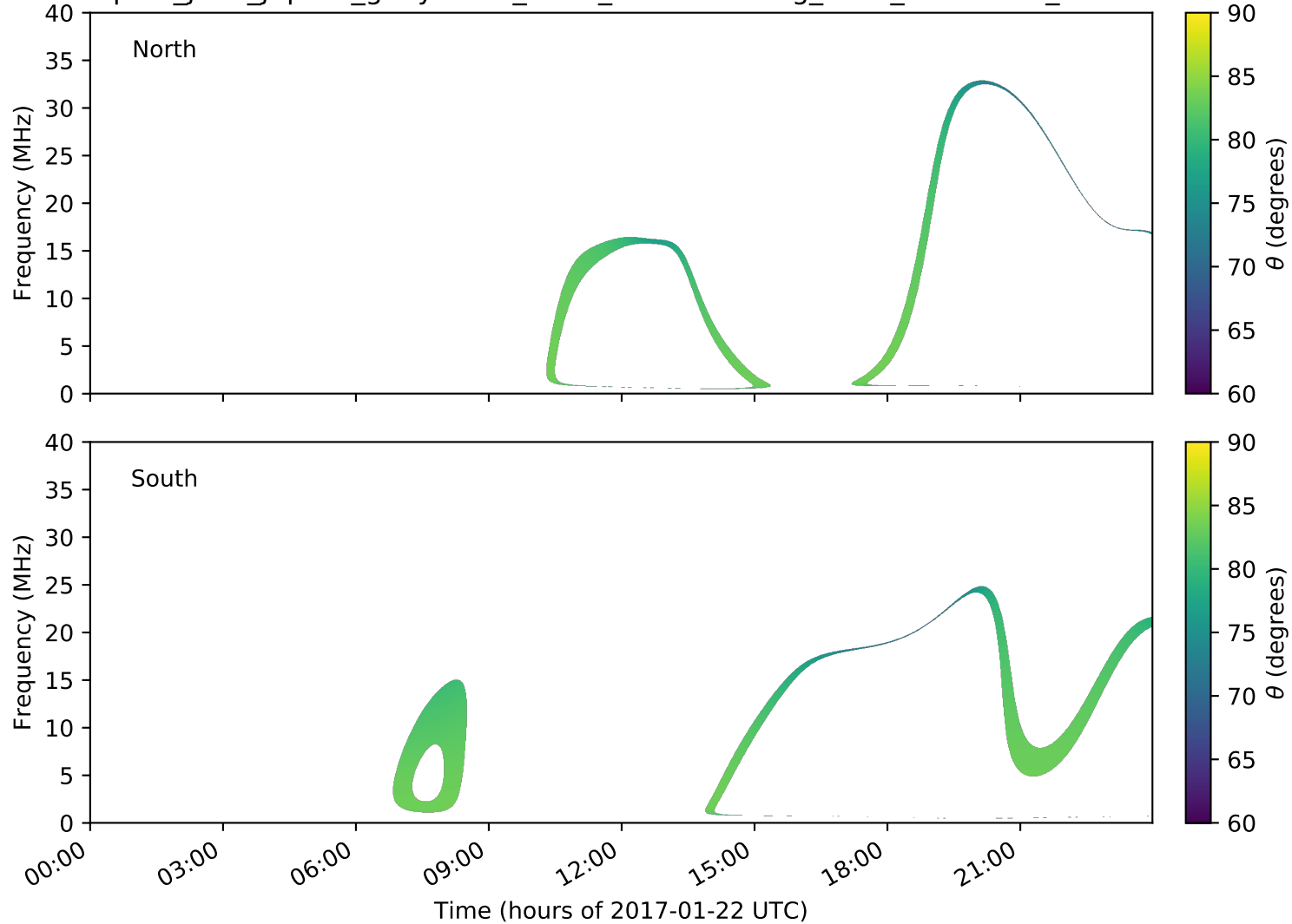
expres_juno_jupiter_ganymede_isaac_lossc-wid1deg_3kev_20170122_v01.cdf
