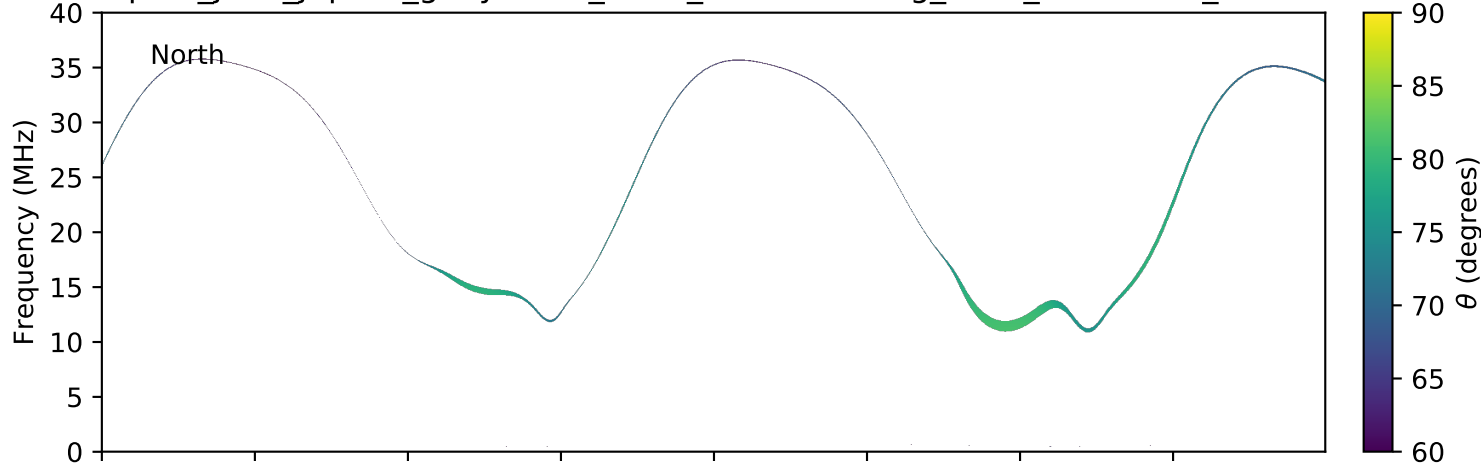
expres_juno_jupiter_ganymede_isaac_lossc-wid1deg_3kev_20170117_v01.cdf
