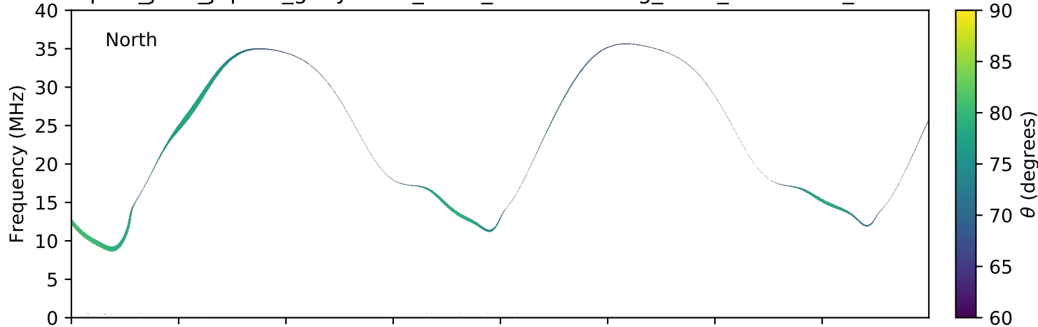
expres_juno_jupiter_ganymede_isaac_lossc-wid1deg_3kev_20170116_v01.cdf
