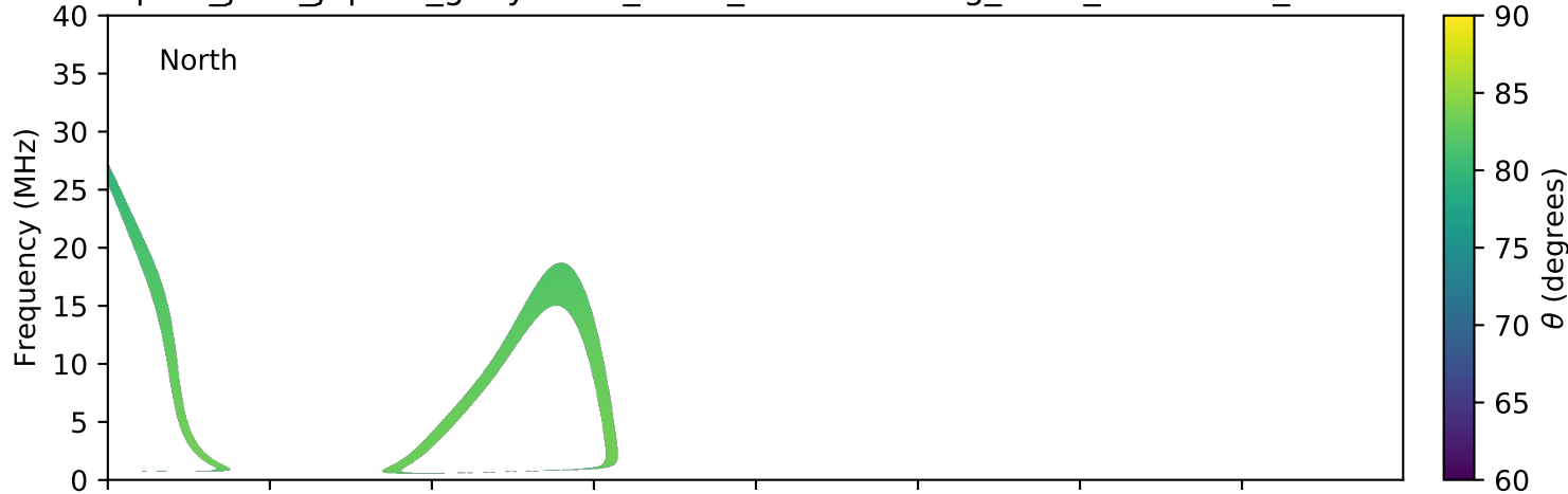
expres_juno_jupiter_ganymede_isaac_lossc-wid1deg_3kev_20170111_v01.cdf
