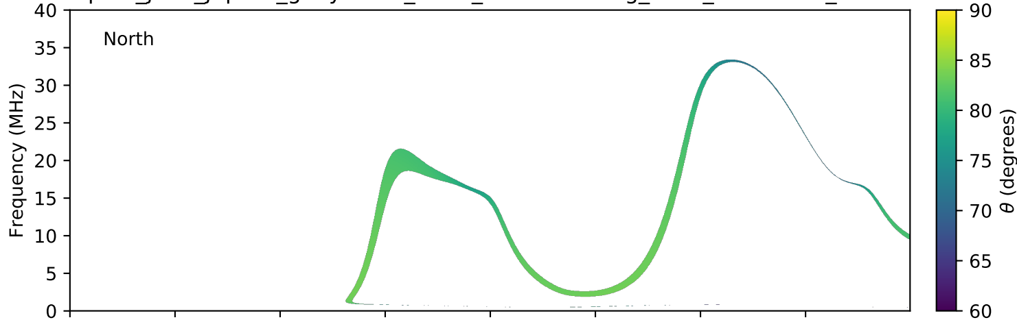
expres_juno_jupiter_ganymede_isaac_lossc-wid1deg_3kev_20170108_v01.cdf
