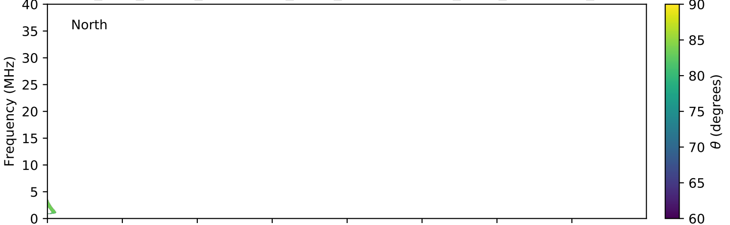
expres_juno_jupiter_ganymede_isaac_lossc-wid1deg_3kev_20170104_v01.cdf
