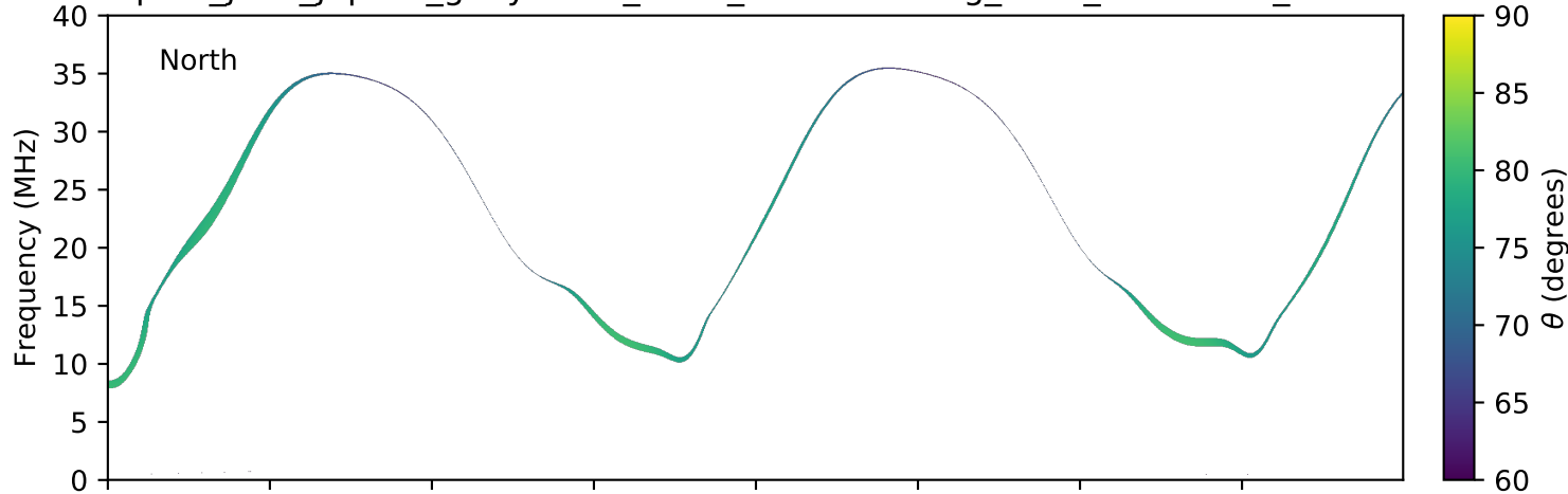
expres_juno_jupiter_ganymede_isaac_lossc-wid1deg_3kev_20170102_v01.cdf
