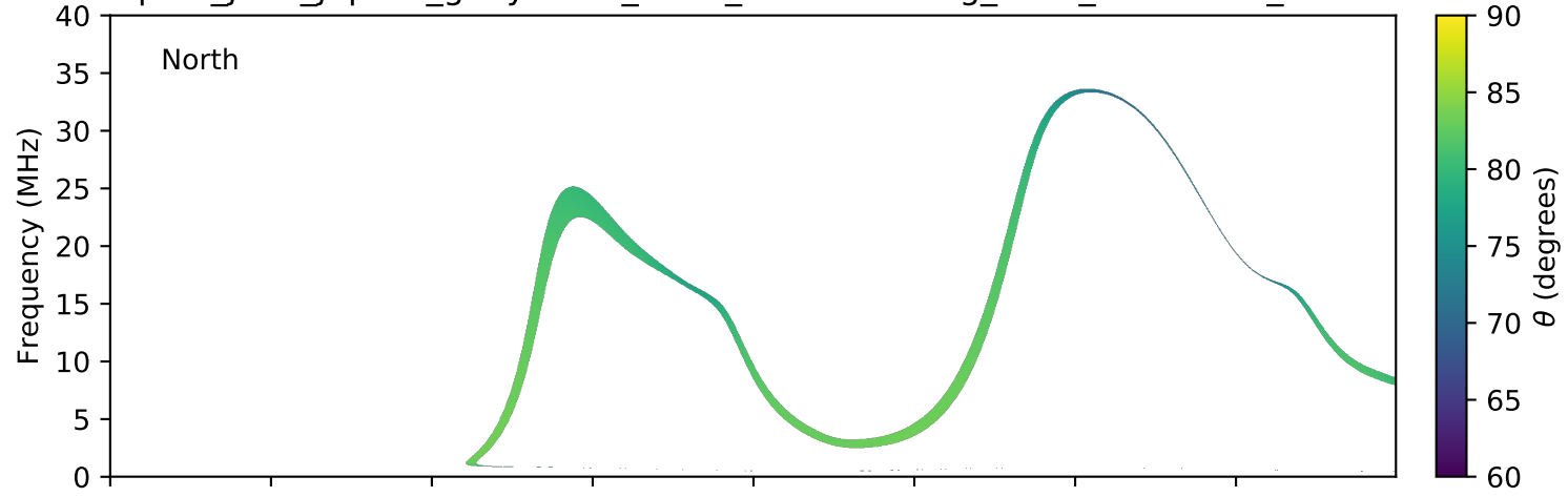
expres_juno_jupiter_ganymede_isaac_lossc-wid1deg_3kev_20170101_v01.cdf
