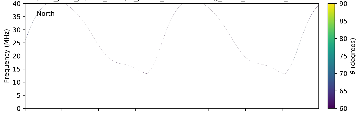
expres_juno_jupiter_europa_jrm09_lossc-wid1deg_3kev_20170131_v01.cdf
