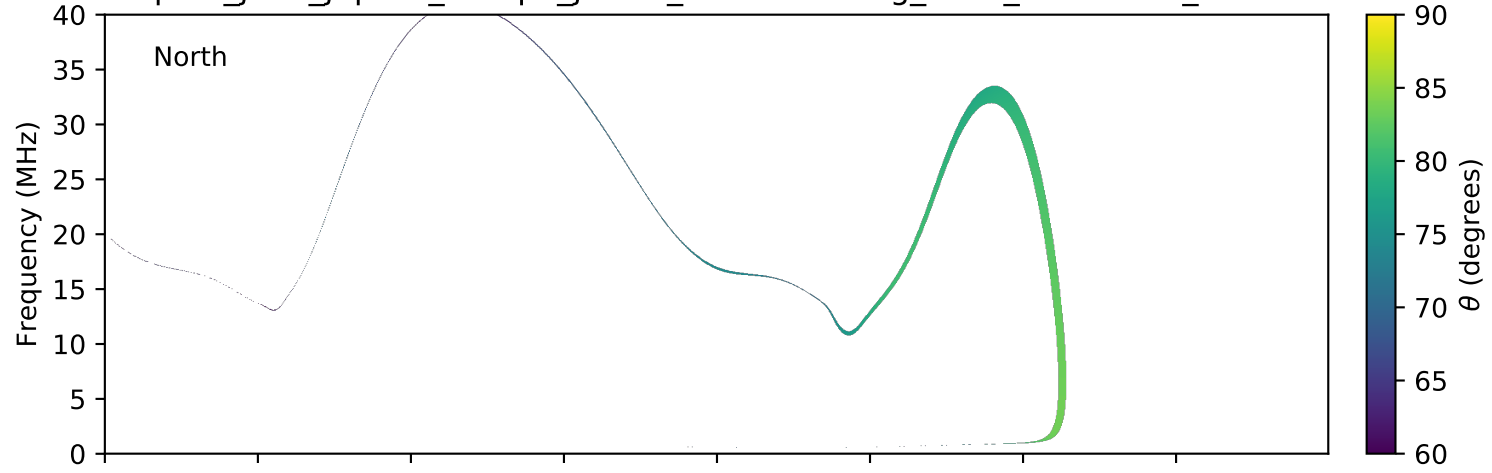
expres_juno_jupiter_europa_jrm09_lossc-wid1deg_3kev_20170128_v01.cdf
