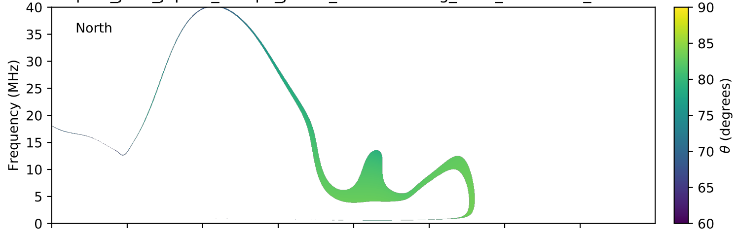
expres_juno_jupiter_europa_jrm09_lossc-wid1deg_3kev_20170121_v01.cdf
