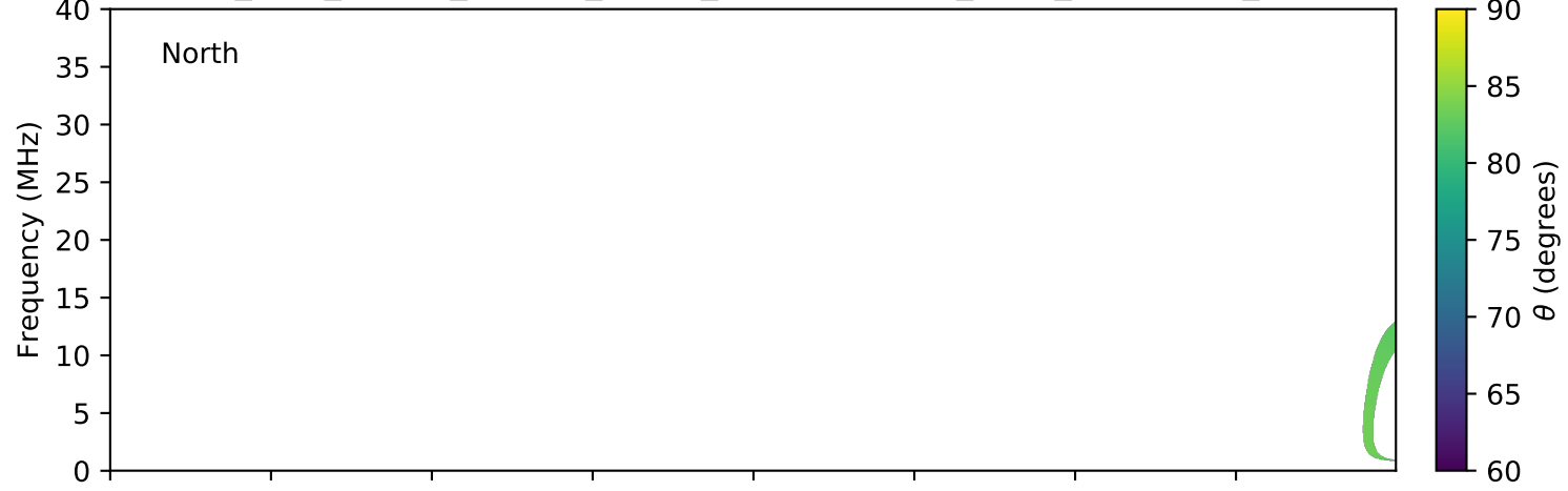
expres_juno_jupiter_europa_jrm09_lossc-wid1deg_3kev_20170119_v01.cdf
