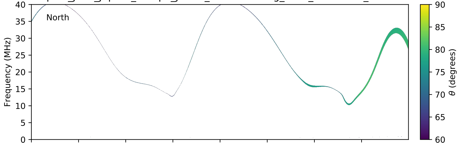
expres_juno_jupiter_europa_jrm09_lossc-wid1deg_3kev_20170117_v01.cdf
