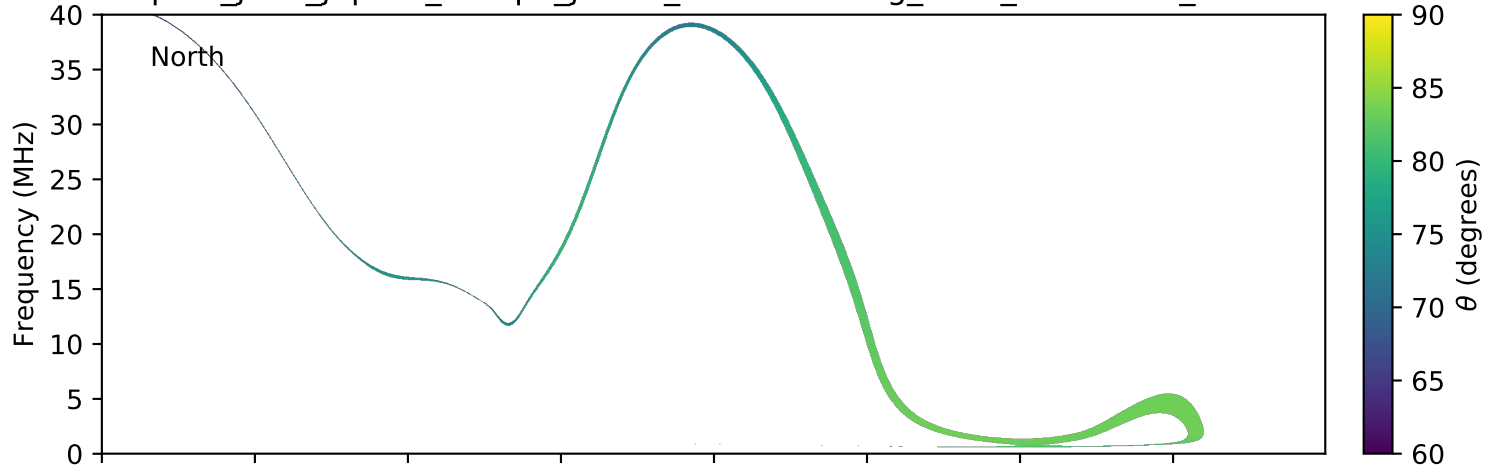
expres_juno_jupiter_europa_jrm09_lossc-wid1deg_3kev_20170103_v01.cdf
