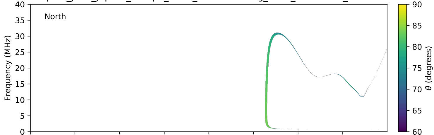
expres_juno_jupiter_europa_isaac_lossc-wid1deg_3kev_20170130_v01.cdf
