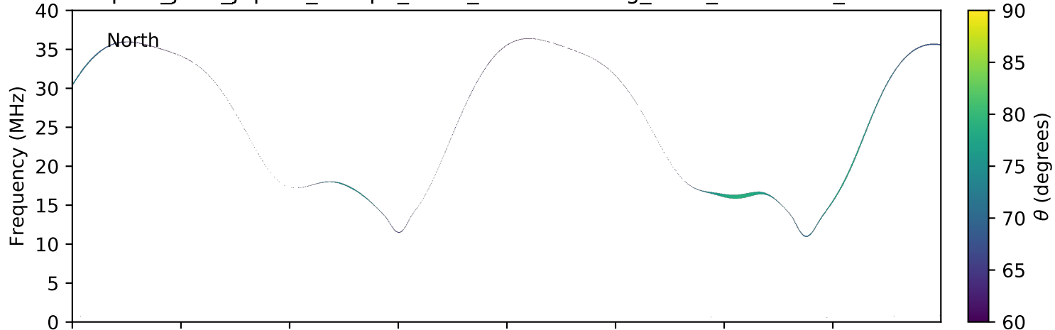
expres_juno_jupiter_europa_isaac_lossc-wid1deg_3kev_20170124_v01.cdf
