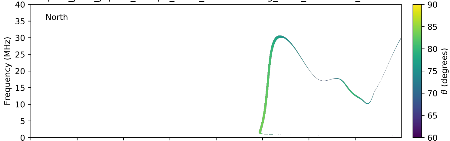
expres_juno_jupiter_europa_isaac_lossc-wid1deg_3kev_20170123_v01.cdf
