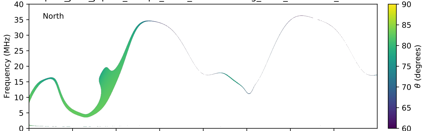
expres_juno_jupiter_europa_isaac_lossc-wid1deg_3kev_20170120_v01.cdf
