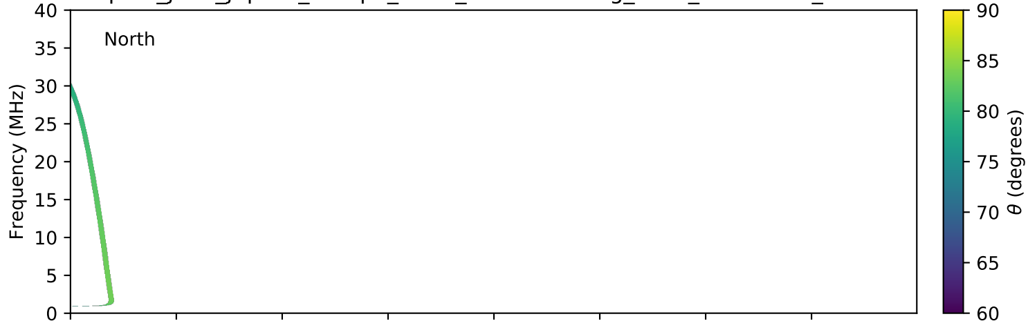
expres_juno_jupiter_europa_isaac_lossc-wid1deg_3kev_20170118_v01.cdf
