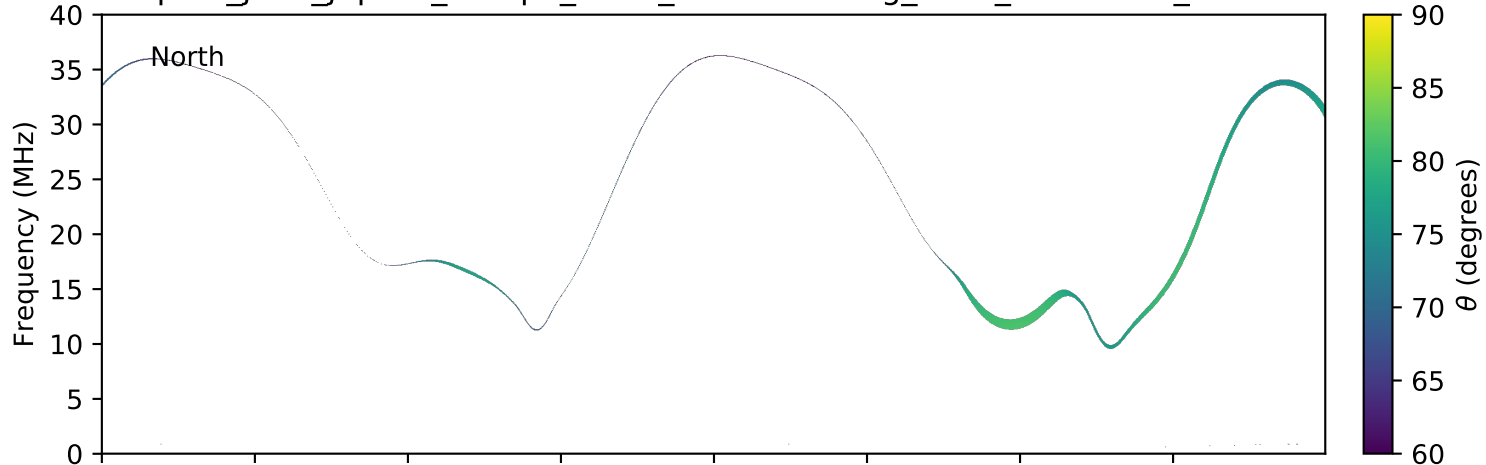
expres_juno_jupiter_europa_isaac_lossc-wid1deg_3kev_20170117_v01.cdf
