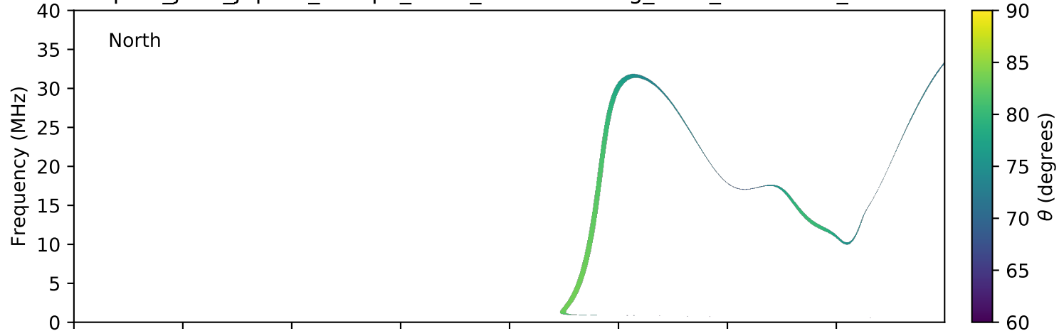
expres_juno_jupiter_europa_isaac_lossc-wid1deg_3kev_20170116_v01.cdf
