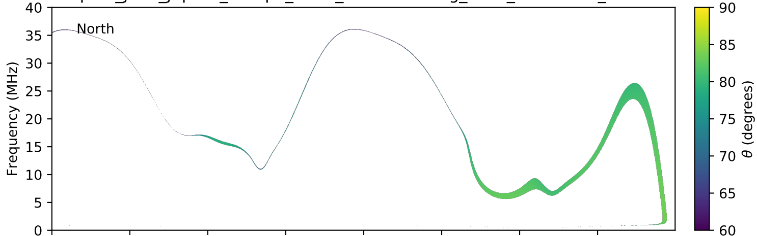
expres_juno_jupiter_europa_isaac_lossc-wid1deg_3kev_20170110_v01.cdf
