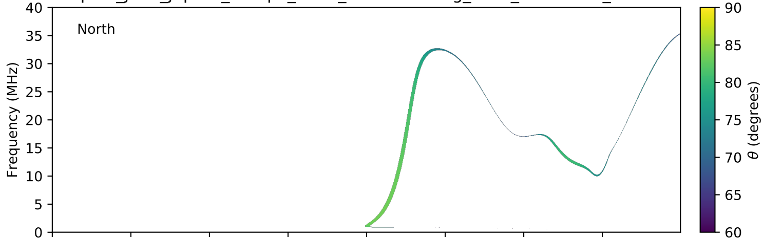
expres_juno_jupiter_europa_isaac_lossc-wid1deg_3kev_20170109_v01.cdf
