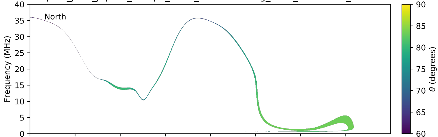
expres_juno_jupiter_europa_isaac_lossc-wid1deg_3kev_20170103_v01.cdf
