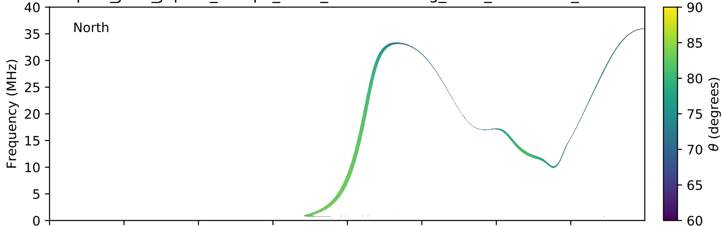
expres_juno_jupiter_europa_isaac_lossc-wid1deg_3kev_20170102_v01.cdf
