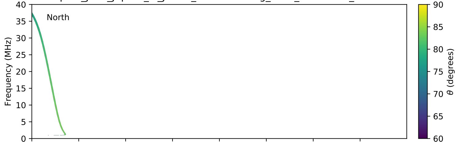
expres_juno_jupiter_io_jrm09_lossc-wid1deg_3kev_20161031_v01.cdf
