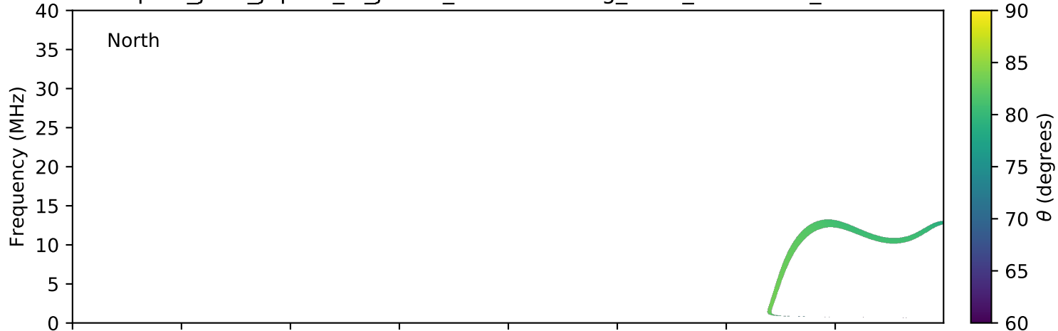
expres_juno_jupiter_io_jrm09_lossc-wid1deg_3kev_20161026_v01.cdf
