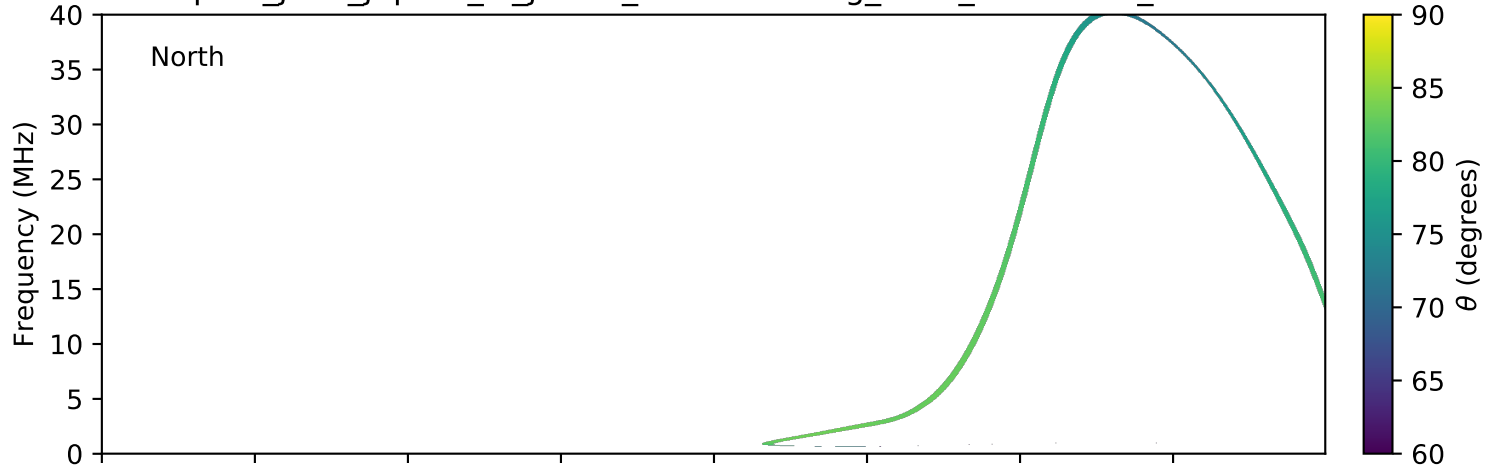
expres_juno_jupiter_io_jrm09_lossc-wid1deg_3kev_20161021_v01.cdf
