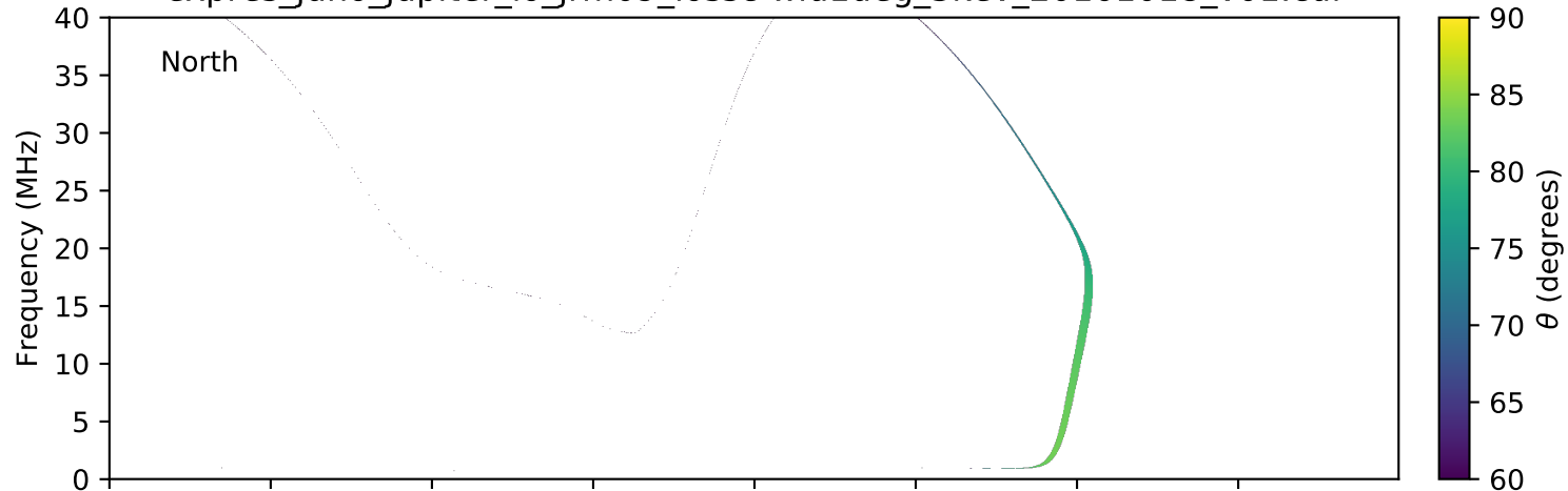
expres_juno_jupiter_io_jrm09_lossc-wid1deg_3kev_20161018_v01.cdf
