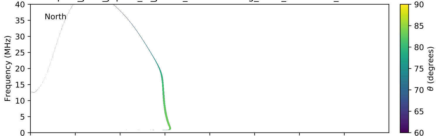
expres_juno_jupiter_io_jrm09_lossc-wid1deg_3kev_20161013_v01.cdf
