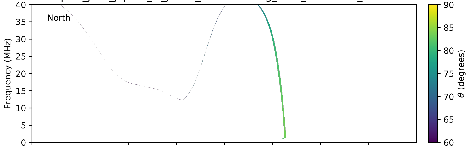
expres_juno_jupiter_io_jrm09_lossc-wid1deg_3kev_20161011_v01.cdf
