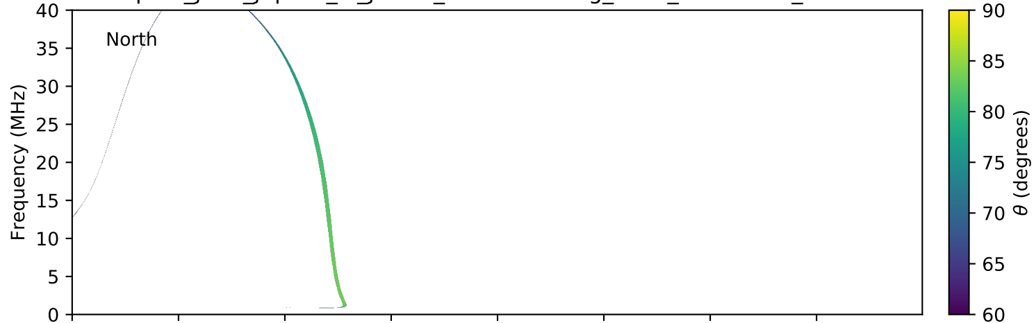
expres_juno_jupiter_io_jrm09_lossc-wid1deg_3kev_20161006_v01.cdf
