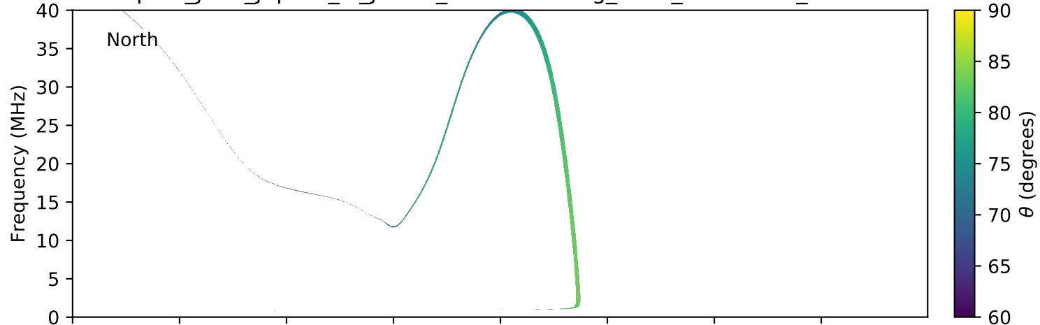
expres_juno_jupiter_io_jrm09_lossc-wid1deg_3kev_20161004_v01.cdf
