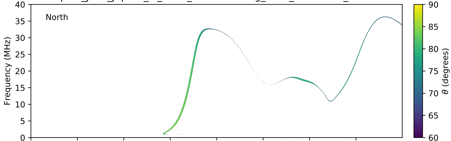
expres_juno_jupiter_io_isaac_lossc-wid1deg_3kev_20161030_v01.cdf
