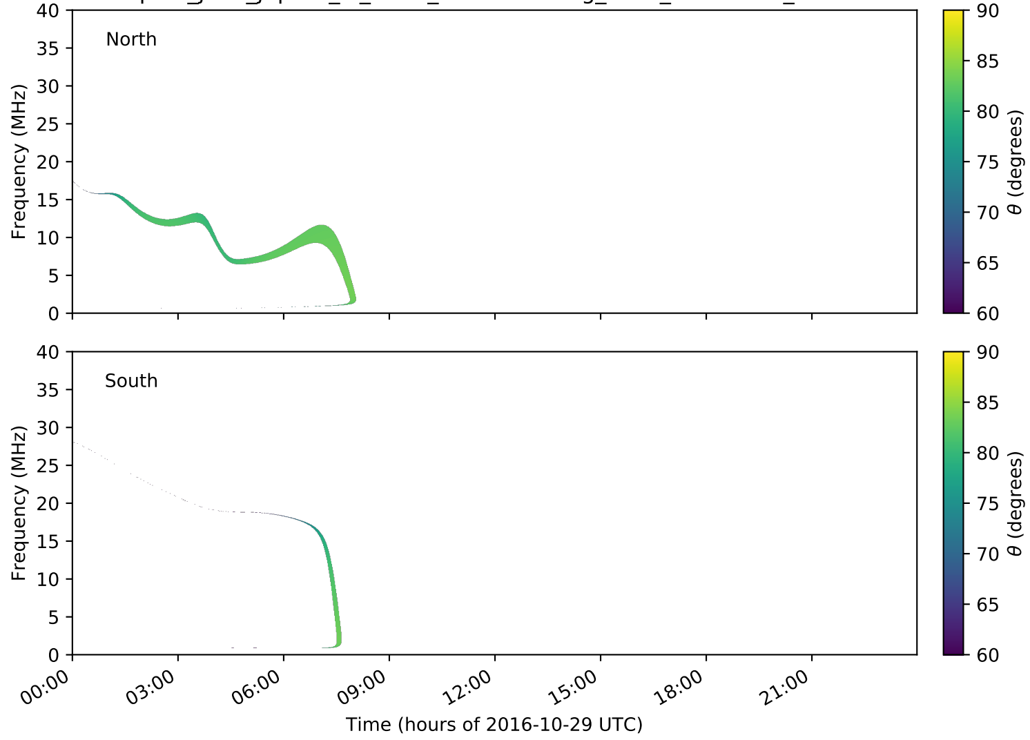
expres_juno_jupiter_io_isaac_lossc-wid1deg_3kev_20161029_v01.cdf
