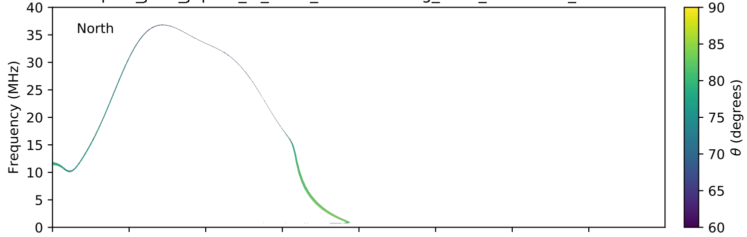
expres_juno_jupiter_io_isaac_lossc-wid1deg_3kev_20161027_v01.cdf
