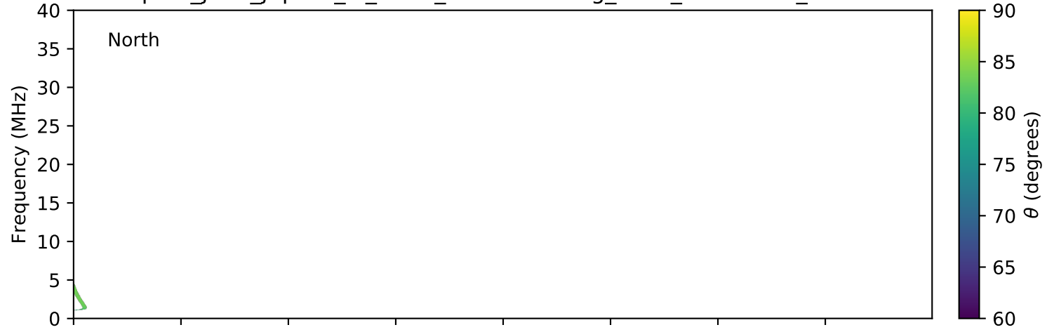
expres_juno_jupiter_io_isaac_lossc-wid1deg_3kev_20161024_v01.cdf
