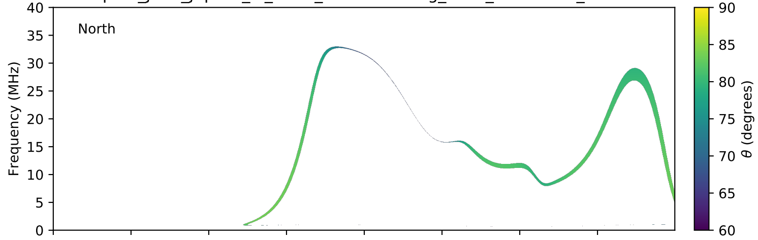
expres_juno_jupiter_io_isaac_lossc-wid1deg_3kev_20161023_v01.cdf
