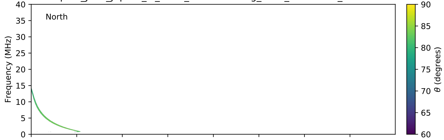
expres_juno_jupiter_io_isaac_lossc-wid1deg_3kev_20161022_v01.cdf
