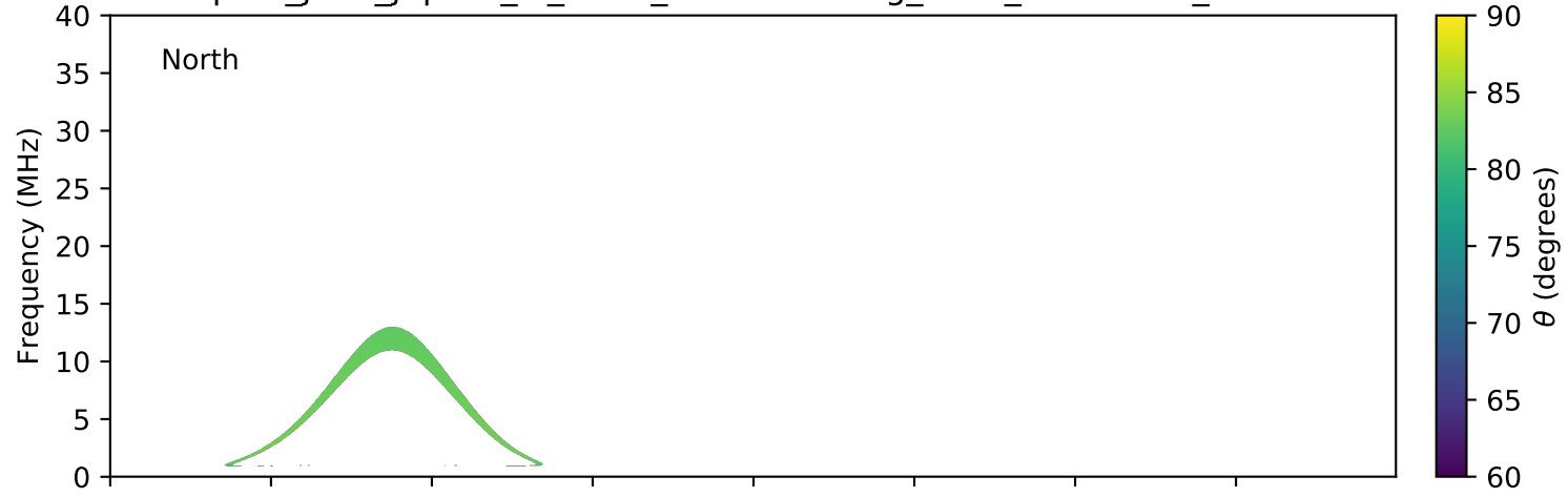
expres_juno_jupiter_io_isaac_lossc-wid1deg_3kev_20161020_v01.cdf
